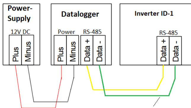
Shielded RS485 Cable. Max Length- 1000m
